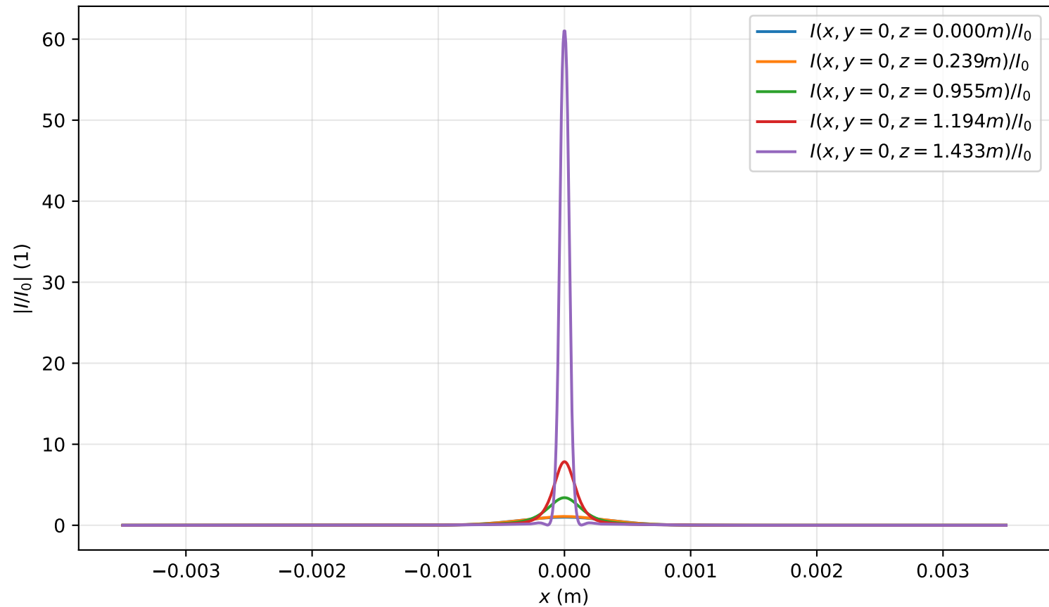
Intensity profile I(x, y = 0, z)/I_0 , Pin=1.7Pcr, artificial time
